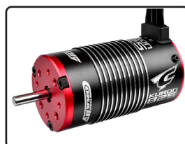
C-54055 Brushless Motor - Kuron 825 - 4-Pole - 2050 KV - Sensorless
