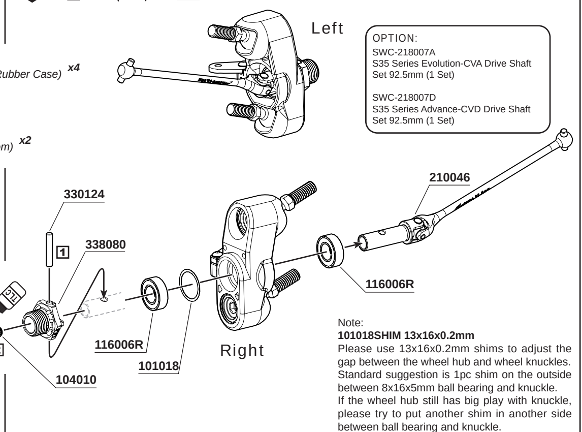
101018 SHIM 13x16x0.2mm x2
