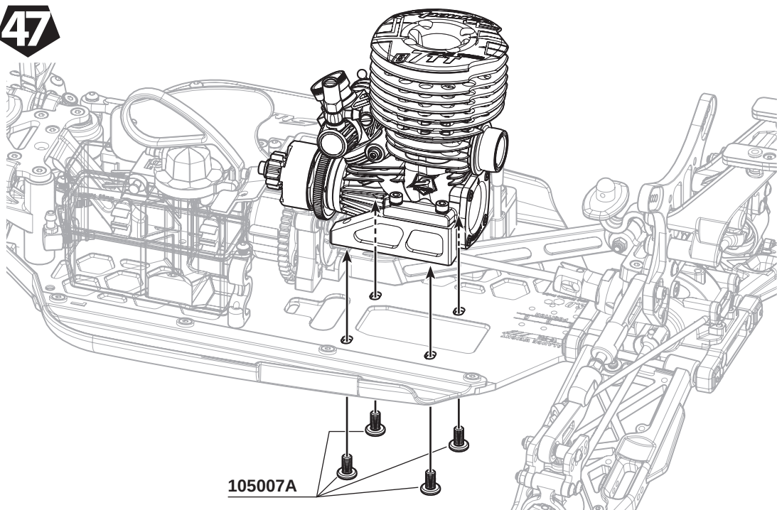
105007A M4x8mm I-Head Screw x4
