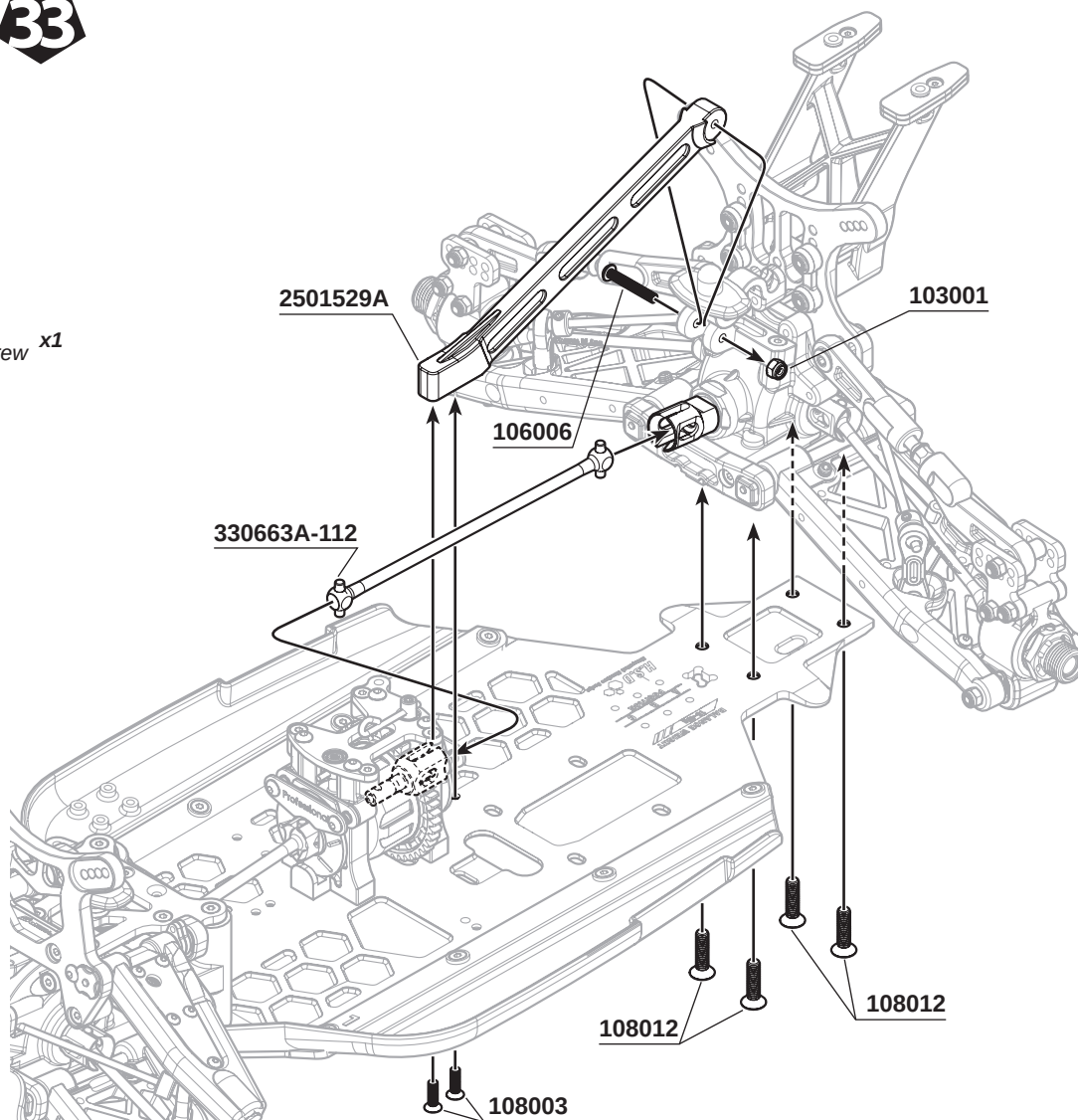
108012 M4x16mm FH/ST HEX Screw x4
