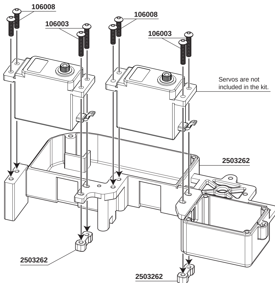
106008 M3x12mm Hex Socket OH/TP Screw x4
