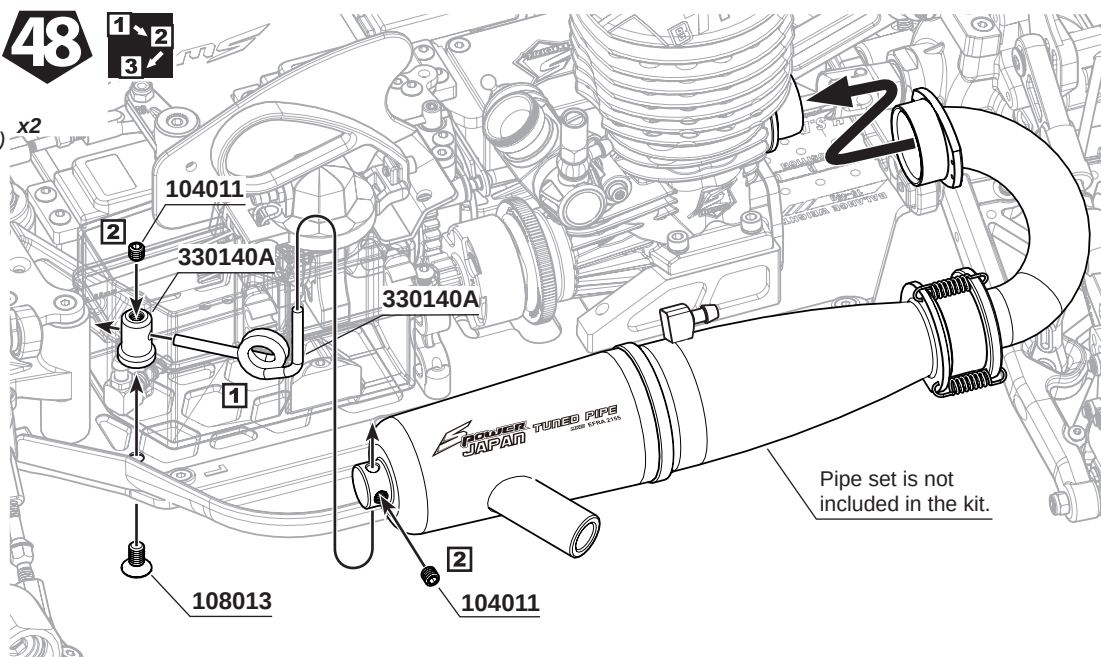
108013 M4x8mm FH/ST HEX Screw x1
