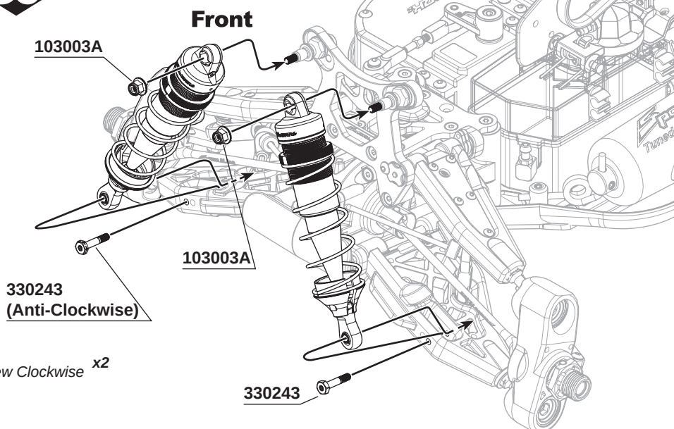
330243 SWORKz 3x16mm Shock Hex Screw Anti-Clockwise x2
