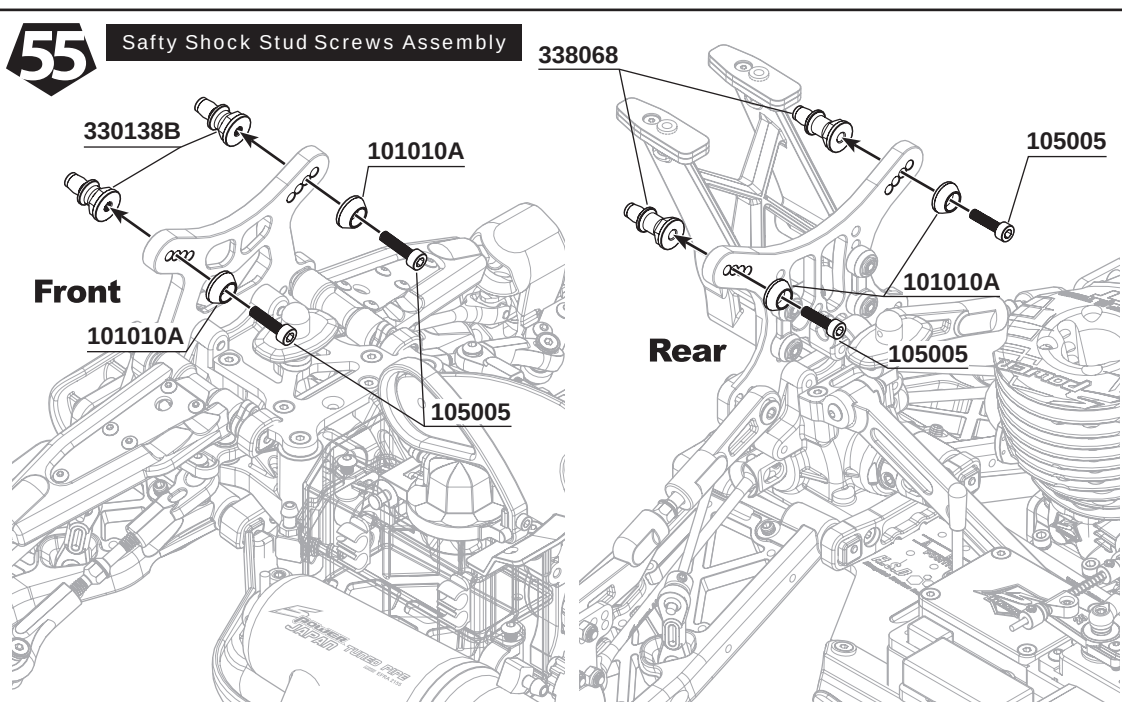
105005 M3x12mm Cap Screw x4
