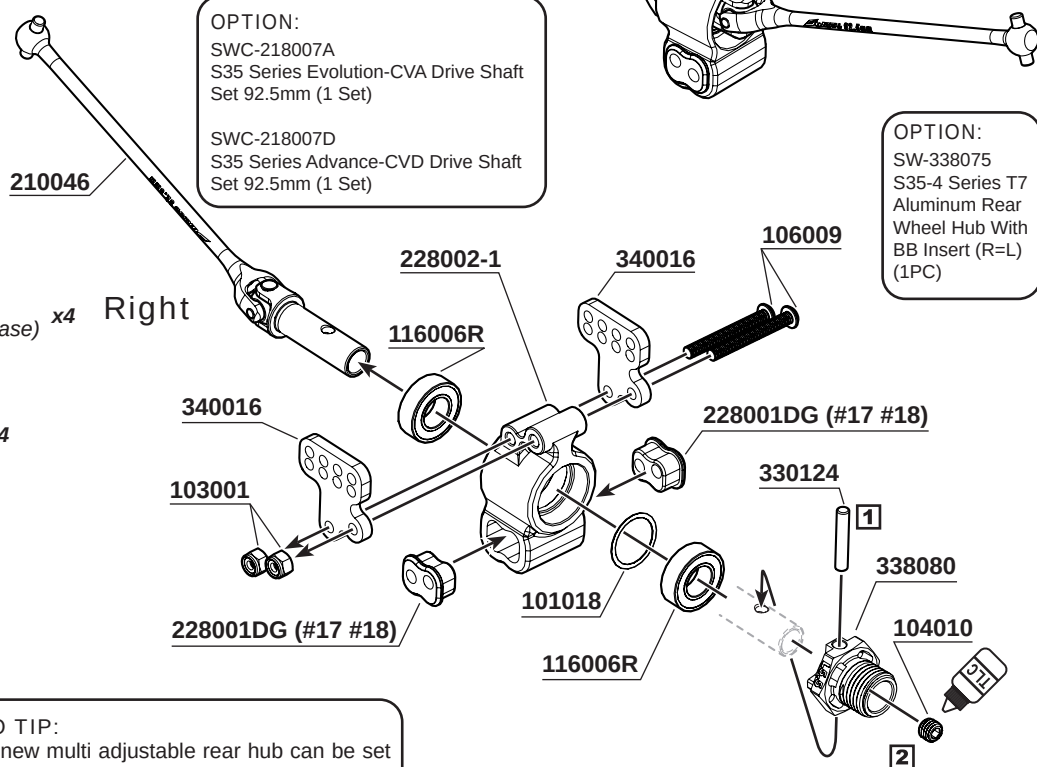
106009 M3x25mm Hex Socket OH/TP Screw x4
