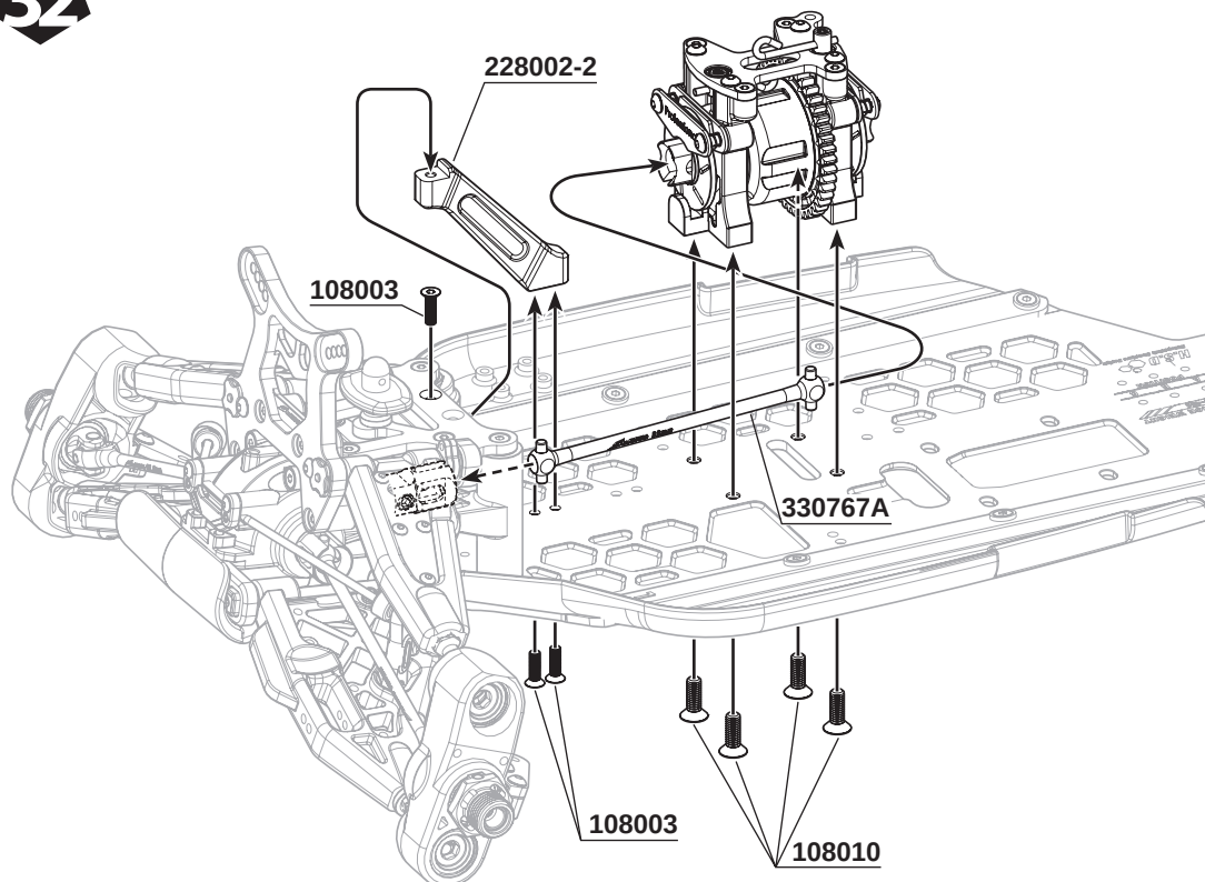
108003 M3x10mm FH/ST HEX Screw x3
