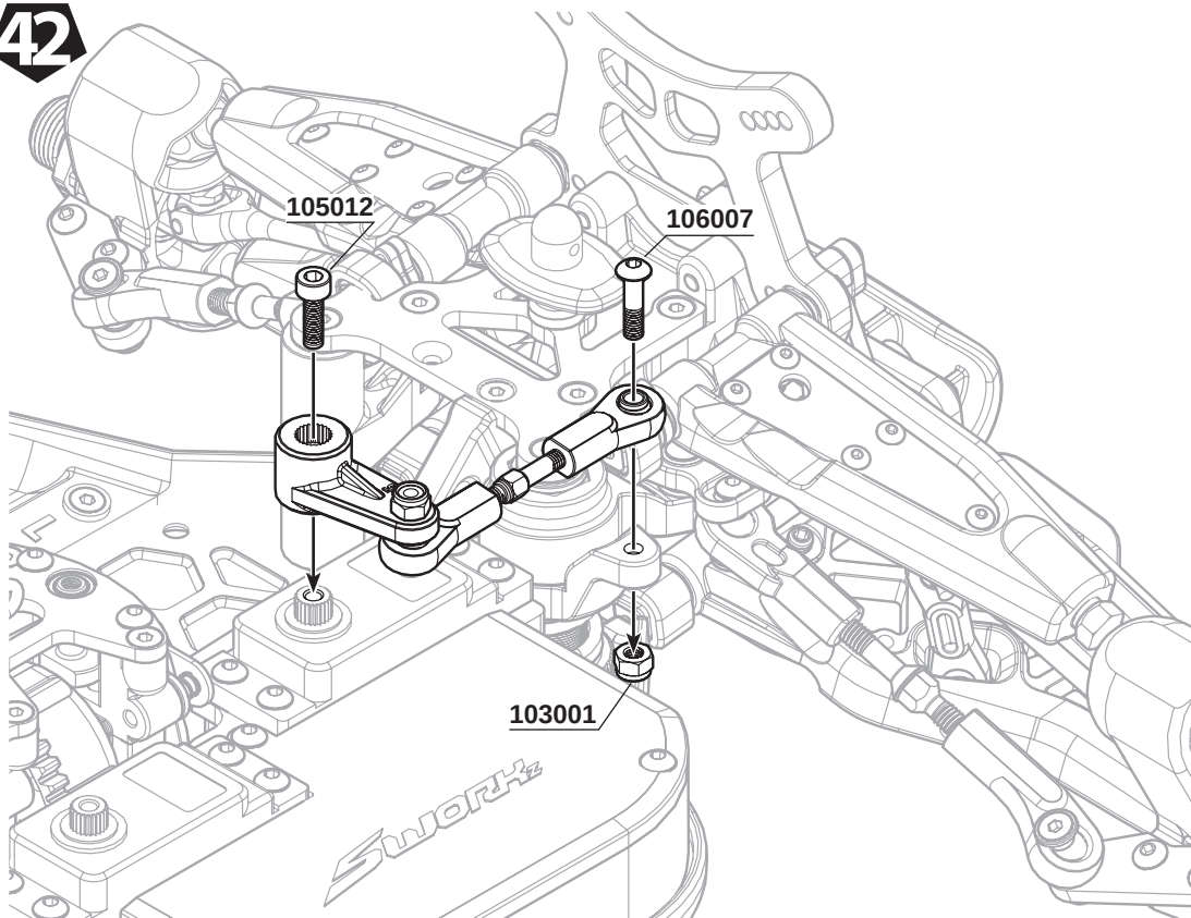
106007 M3x12mm Hex Socket OH/TP Screw (HT) x1
