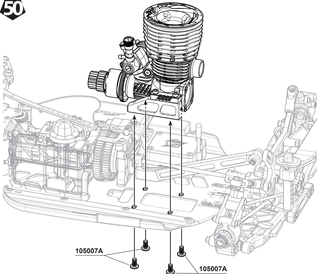
105007A M4x8mm I-Head Screw x4
