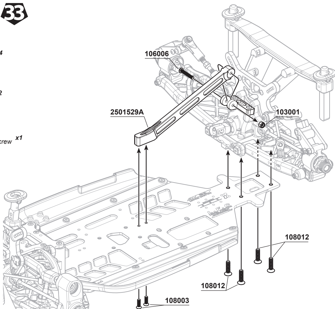
108003 M3x10mm FH/ST HEX Screw x2
