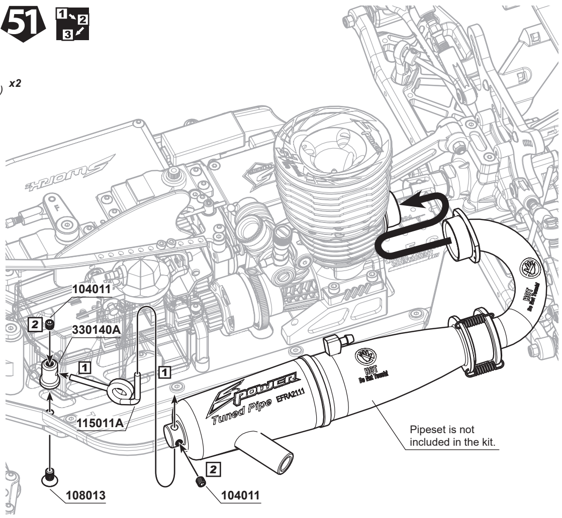
108013 M4x8mm FH/ST HEX Screw x1
