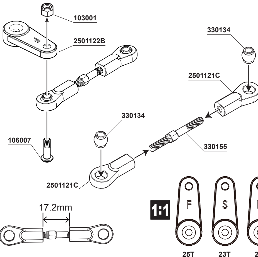
106007 M3x12mm Hex Socket OH/TP Screw(HT) x1
