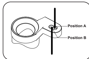
SW-338052 S35-4 Series T7 Aluminum Setting Bellcrank Upper Part-A (with 2Hole )
