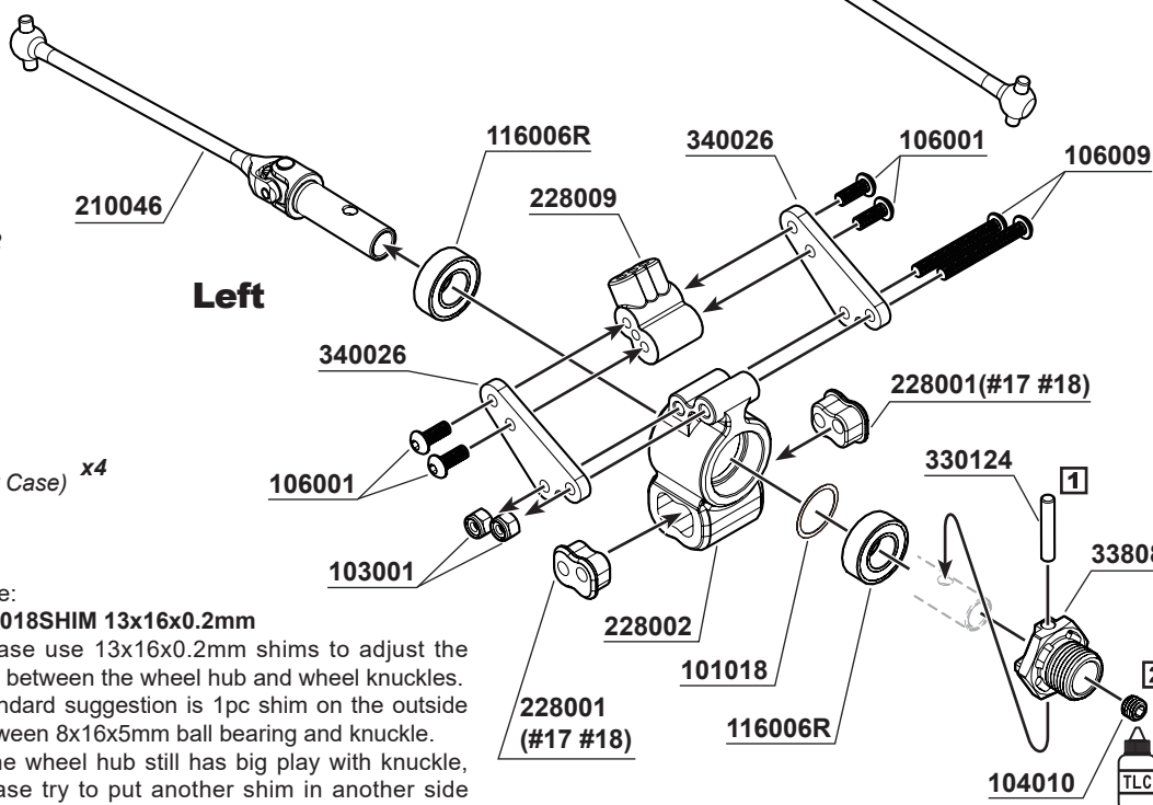
104010 M5x4mm Set Screw (Flat Bottom) x2
