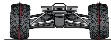
Negative camber
