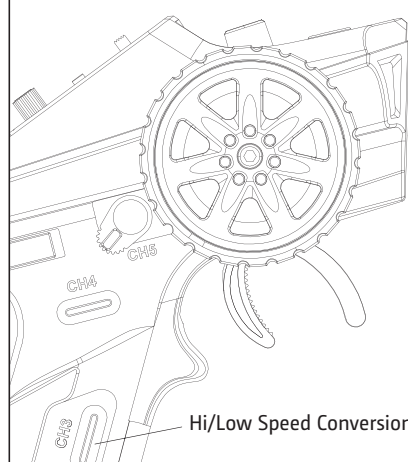
CH3 high-low speed shift switch. When the indicator is off, the gearbox is in the high-speed mode.
