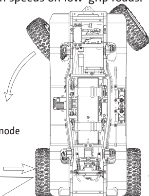
In this mode, the rear left wheel is locked/braked when turn left
