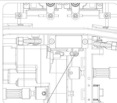
CH3 high-low speed shift switch. When the indicator is off, the gearbox is in the high-speed mode.
