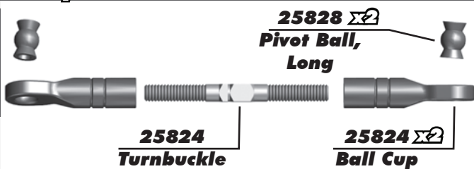
Steering Turnbuckle 22.00mm
