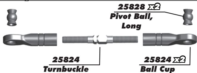
Steering Turnbuckle 15.50mm
