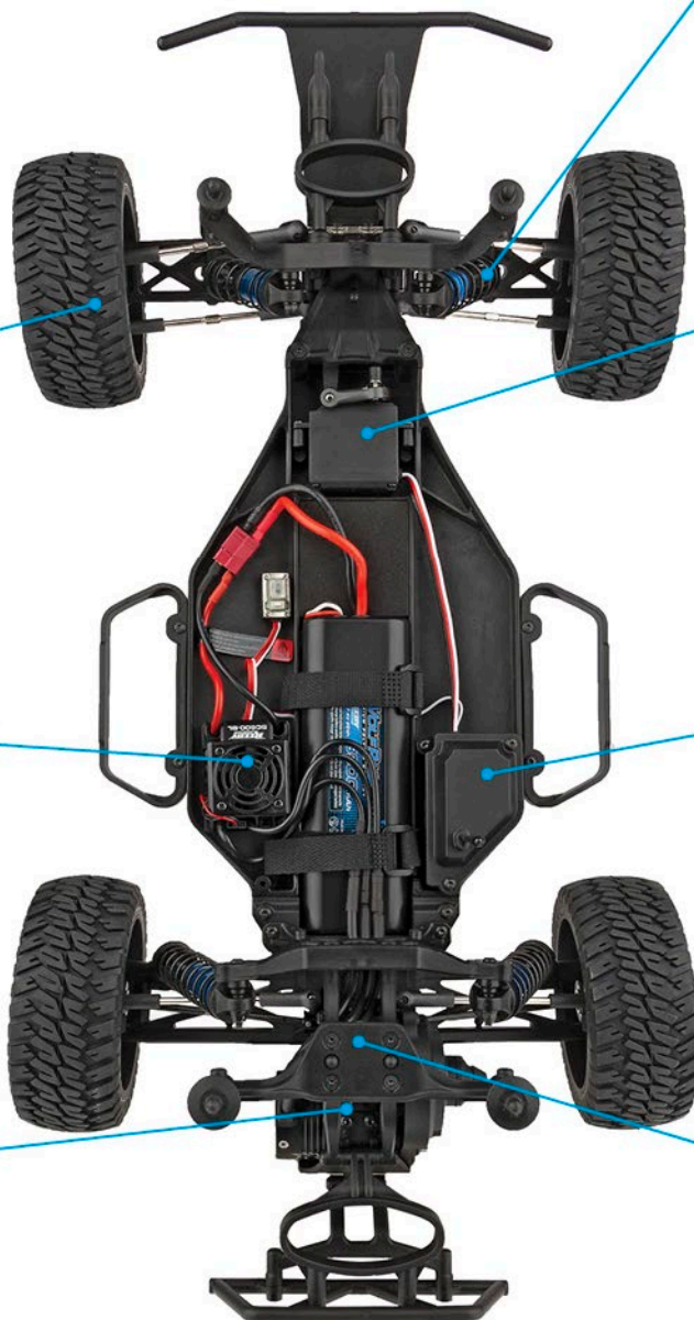
Water-resistant, Reedy brushless electronic speed controller with High Current T-Plug
