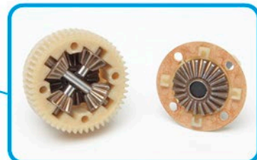
2.6:1 ratio gearbox with heavy-duty, sealed gear differential
