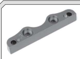
67384 Front Suspension Block (FR) - 7075
