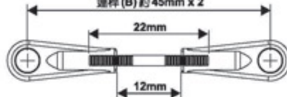
Linkage rod (B) Approx. 45mm x 2 連桿 (B) 約 45mm x 2
