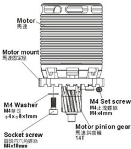
Socket screw 圓頭內六角螺絲 (M4x10mm) x 4
