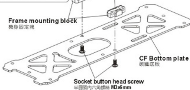
Socket button head screw 半圓頭內六角螺絲 (M3x6mm) x 2
